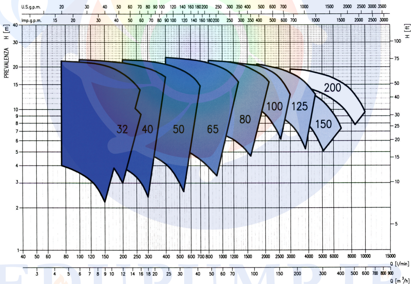
PERFORMANCE CHART MMD4 SERIES 4 POLES
