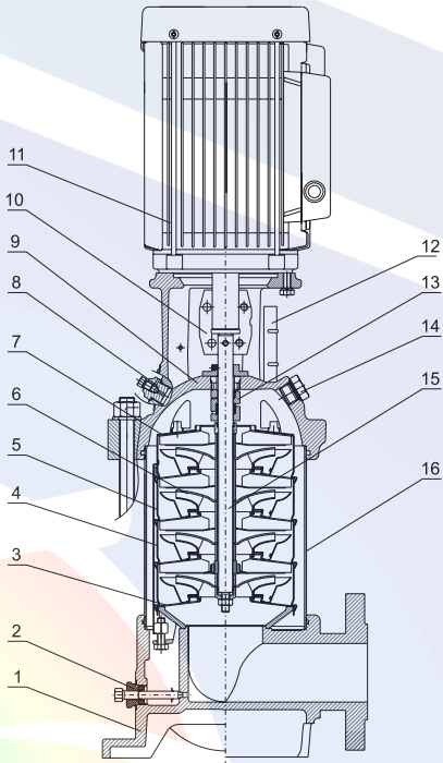
MODEL: LVR10(15,20)
