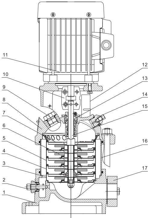
MODEL: LVR1(2,3,4,5)
