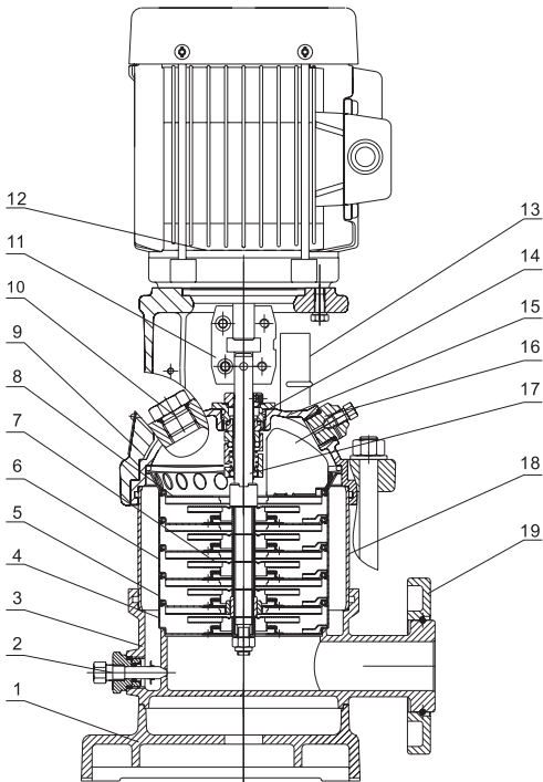
MODEL: LVS1(2,3,4,5)
