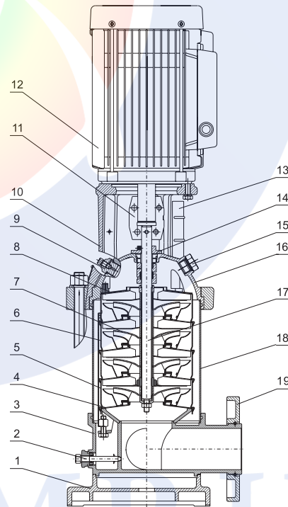
MODEL: LVS10(15,20)
